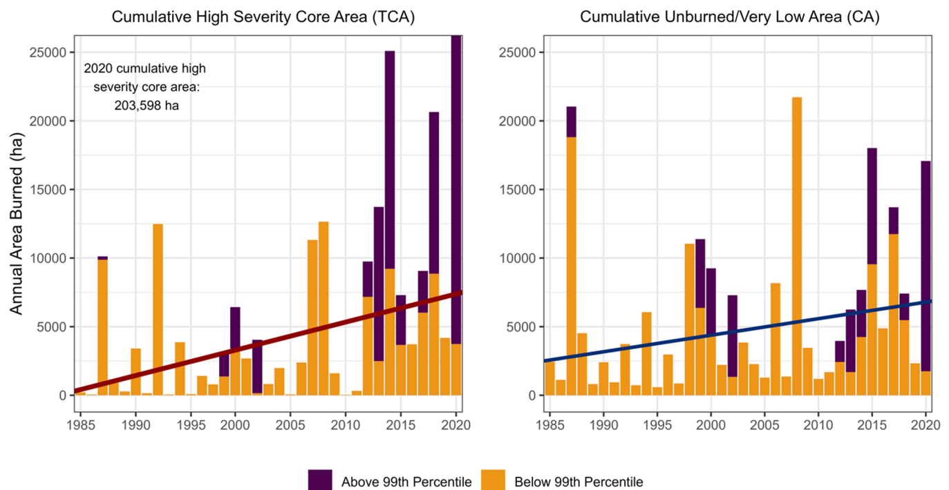
Fig. 6. Trends in total annual interior core area of high severity (TCA, left panel) and total annual unburned refugia-very low severity (CA, right panel) between 1985 and 2020 across the study area. Trend lines represent Theil-Sen slope estimations of high-severity core area (left panel, red line) and total unburned area (right panel, blue line). Note that for the year 2020, total core area burned at high severity (left panel) extends beyond the y-axis limits; the total amount is noted at the top left of the plot. (For interpretation of the references to colour in this figure legend, the reader is referred to the web version of this article.)
