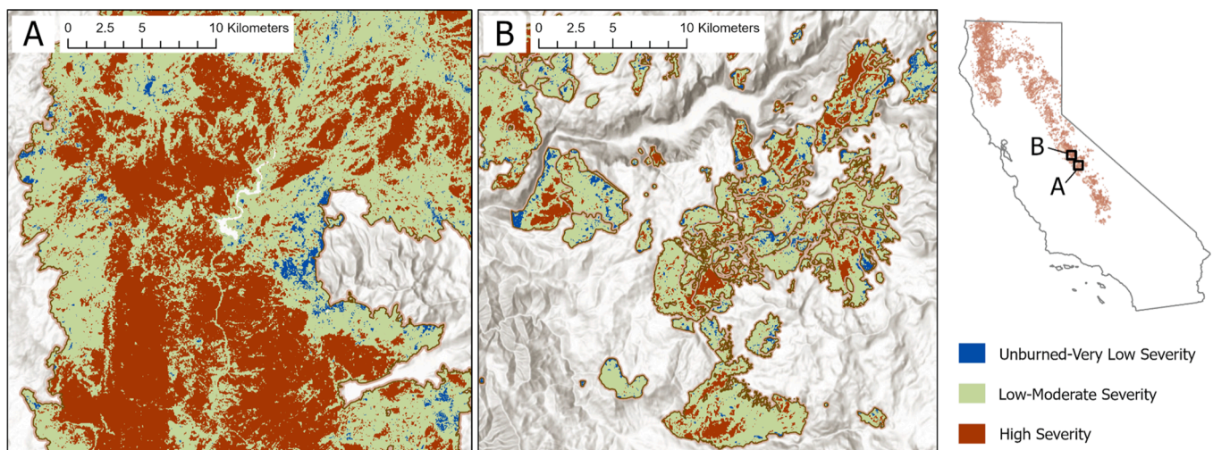
Fig. 7. Impacts of one exceptionally large fire (Panel A, left) versus dozens of smaller fires (Panel B, right) on California forests. Panel A shows the 2020 Creek Fire in the Sierra Nevada, which contains some of the largest single patches of high and low-moderate severity (greater than 20,000 ha) in this analysis. Panel B shows a mosaic of 80 small fires ranging from 4 ha to 3,470 ha that burned between 1985 and 2020 just south of Yosemite Valley in the Sierra Nevada. In both panels, dark blue represents unburned-very low severity, light green represents low-moderate severity, and dark red represents high severity. Both panels are at the same spatial scale and have the same areal extent. (For interpretation of the references to colour in this figure legend, the reader is referred to the web version of this article.)
