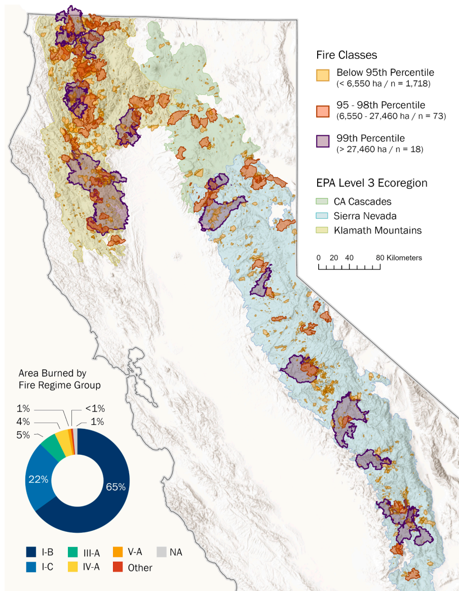
Fig. 1. Map of the study region in California, USA showing locations of 1,809 fires that burned in predominantly conifer forests between 1985 and 2020 in the Klamath (yellow-green), Cascades (green), and Sierra Nevada (blue) EPA Level III ecoregions (Omernik & Gallant, 1987). Spatial patterns of fires were analyzed by their size class: fires below the 95th percentile by size (light orange), fires between the 95th and 98th percentile by fire size (red orange), and exceptionally large 99th percentile fires by size (purple). The majority (87%) of area burned within our study area is concentrated in historically low-to-moderate, frequent fire regimes (LANDFIRE, 2020). Additional regime types in our study area are found primarily as dispersed pixels, mainly in riparian areas and on north-facing slopes. The graph at the bottom left shows the distribution of burned area across the study area and study period by LANDFIRE Fire Regime Groups: I-B: Percent replacement fire less than 66.7%, fire return interval 6–15 years (65% of the study area); I-C: Percent replacement fire less than 66.7%, fire return interval 16–35 years (22% of the study area); III-A: Percent replacement fire less than 80%, fire return interval 36–100 years (5% of the study area); IV-A: Percent replacement fire greater than 80%, fire return interval 36–100 years (4% of the study area); V-A: Any severity, fire return interval 201–500 years (1% of the study area). The “Other” category captures a range of fire regime types but accounts for less than 1% of the study area. An additional 1% of the study area is classified as “Not Applicable” due to sparse or no vegetation cover. (For interpretation of the references to colour in this figure legend, the reader is referred to the web version of this article.)
