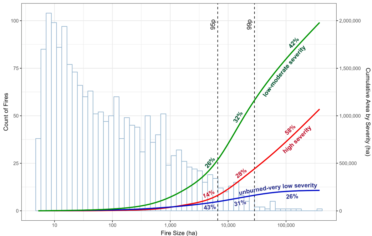
Fig. 3. Histogram of fires by size (left y-axis) for 1,809 fires that burned across conifer-dominated forests in California between 1985 and 2020. Lines represent the cumulative area burned (right y-axis) by severity class (CA), where the bottom blue line is unburned-very low severity, the middle red line is high severity, and the top green line is low-moderate severity. The dashed lines represent the 95th percentile and 99th percentile cutoffs of fires by size. (For interpretation of the references to colour in this figure legend, the reader is referred to the web version of this article.)
