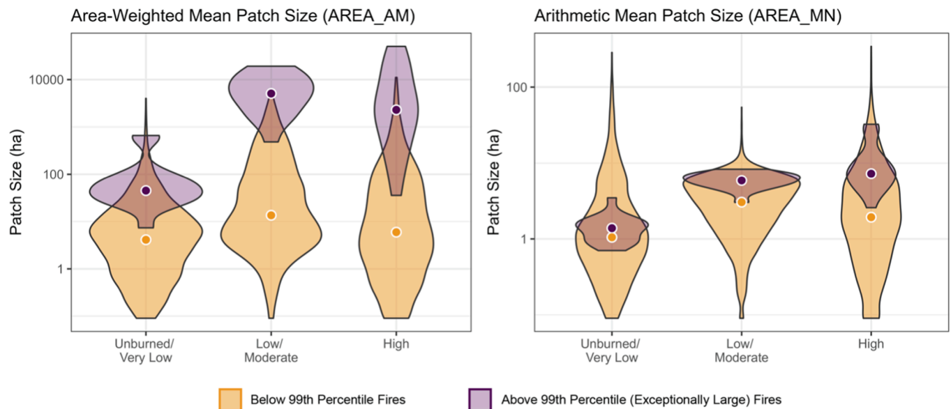
Fig. 5. Distributions of area-weighted mean patch size (AREA_AM, left) and arithmetic mean patch size (AREA_MN, right) by fire for unburned-very low, low-moderate, and high-severity classes as a function of fire size.
