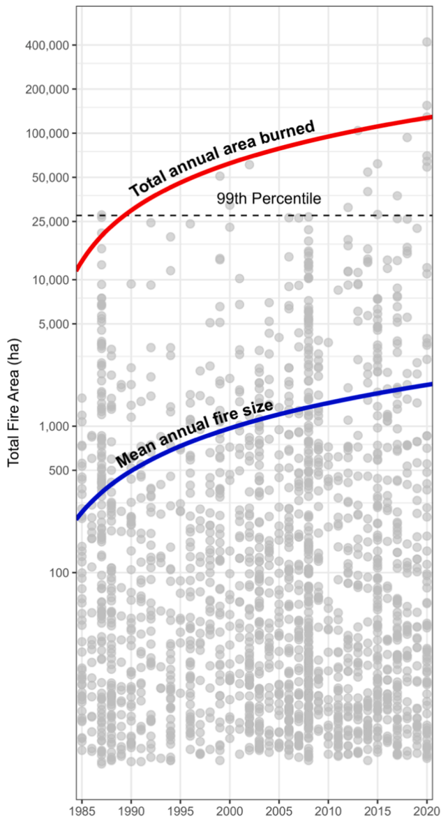
Fig. 2. Trends in mean annual fire size (blue line) and total annual area burned (red line) per Theil-Sen slope estimators. Each gray dot represents a single fire in the corresponding year. The dashed line represents the cutoff of 99th percentile of fires (exceptionally large fires) by size. Trends in mean annual fire size and total annual area burned are statistically significant. (For interpretation of the references to colour in this figure legend, the reader is referred to the web version of this article.)
