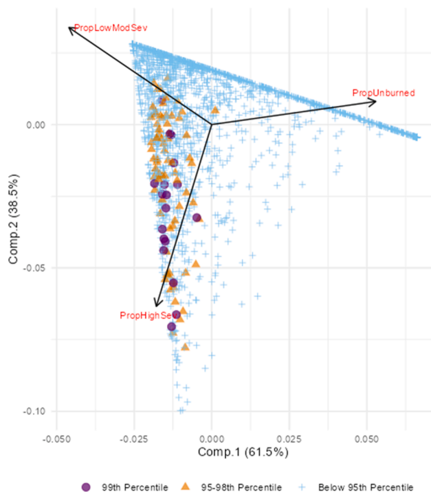
Fig. 4. Ordination of principal component analysis (PCA) of proportional area burned (PLAND) by fire severity class. Fire size groups are overlaid on the plot to show the range of spatial patterns of fire severity in exceptionally large fires ( n = 18 ) and fires between the 95th and 98th percentiles by size. The threshold line of solid points at the top of the ordination represents smaller fires with proportionally greater area unburned.
